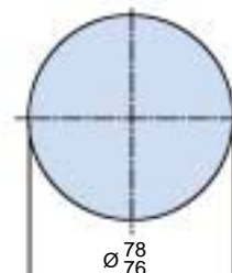
TANK MOUNTING HOLE
