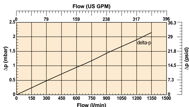
Pressure Loss Curve ABL1
