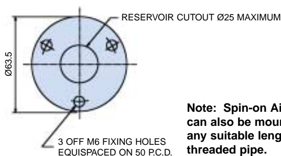
PRESSURISED SPIN-ON AIR BREATHER STEM
