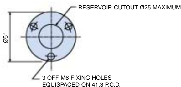
STANDARD SPIN-ON AIR BREATHER STEM
