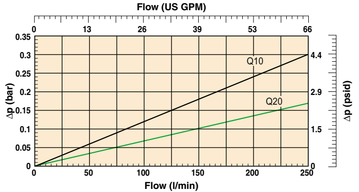
Delta P Clean Element
