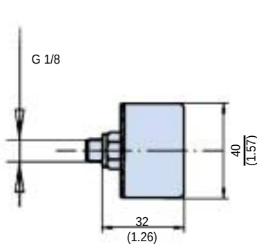
Visual Pressure Indicator Code M10
