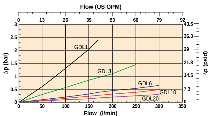
Filter Element TXW4
