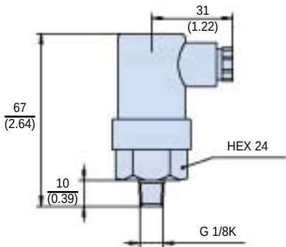
48 VDC Electrical Indicator 1.0 bar Code H10
