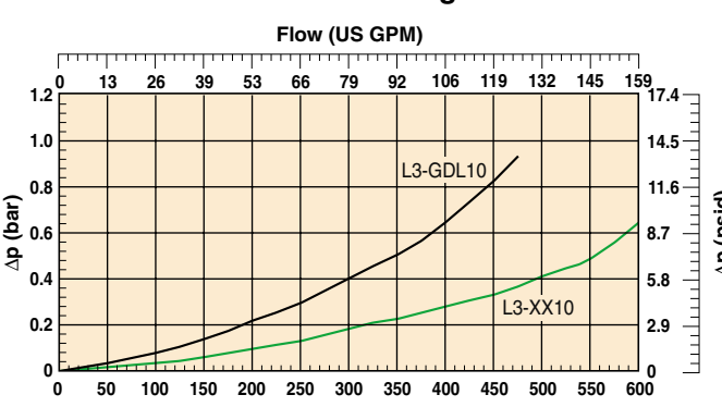
MFA Size 3 Length 3
