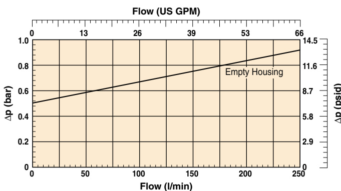
Filter Housing SR2 Without Element
