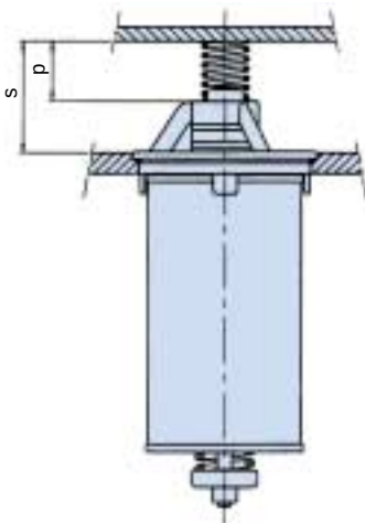
MOUNTING ARRANGEMENT
