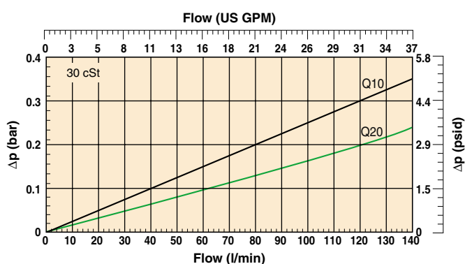
Filter Elements Only \Delta p
