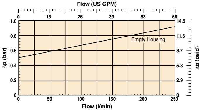
Filter Housing SR2 Without Element
