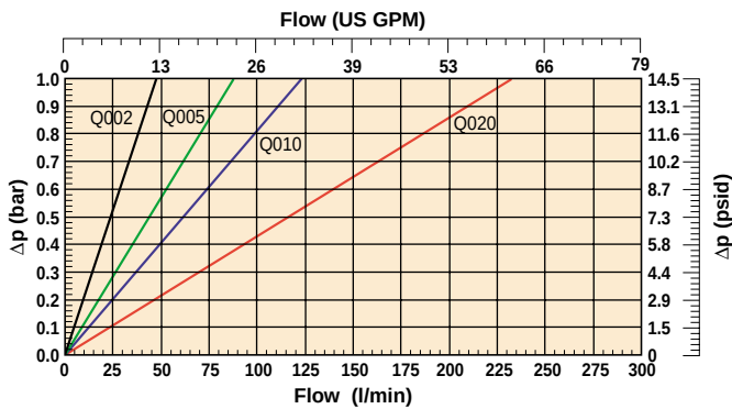
1240 Series with Microglass III Elements
