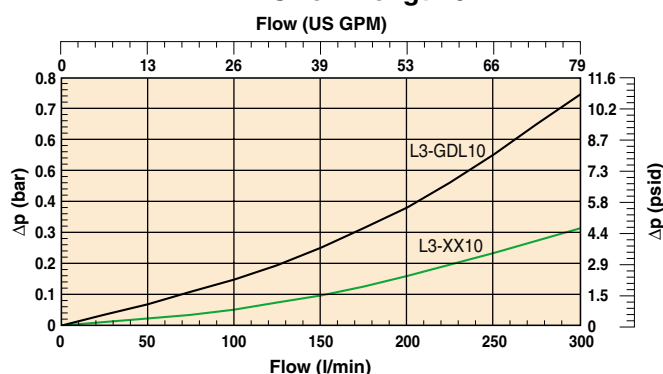
MFL Size 3 Length 3
