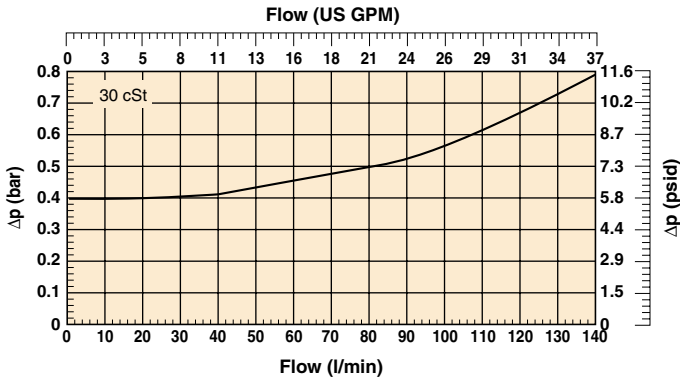
Filter Housing (Without Element) \Delta p
