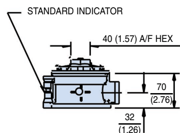
SIZE 2 LENGTH 3
